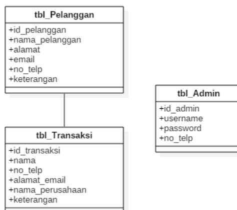
Gambar 3. Class Diagram E-CRM
