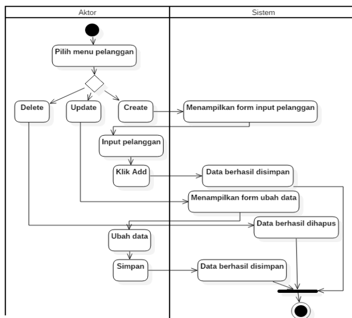
Gambar 2. Activity Diagram Kelola Data Pelanggan
