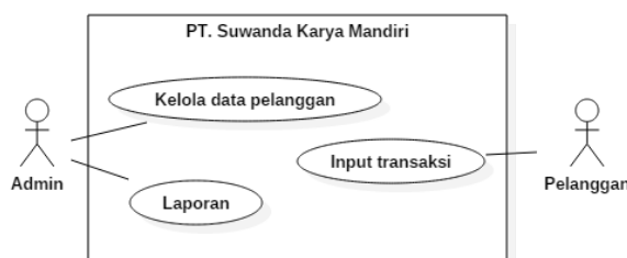
Gambar 1. Use Case Diagram E-CRM
